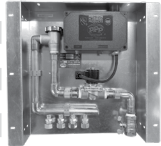
(FLUSH MOUNT)
