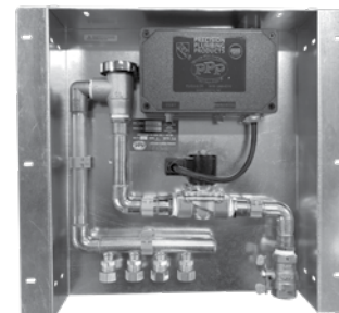
(FLUSH MOUNT)
