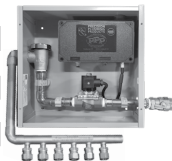
(SURFACE MOUNT)
